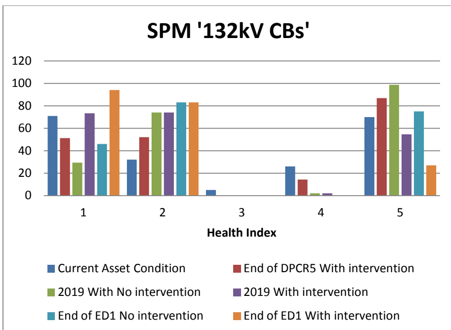
132kV Circuit Breakers
