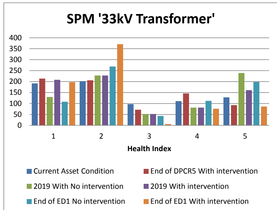
33kv Transformers
