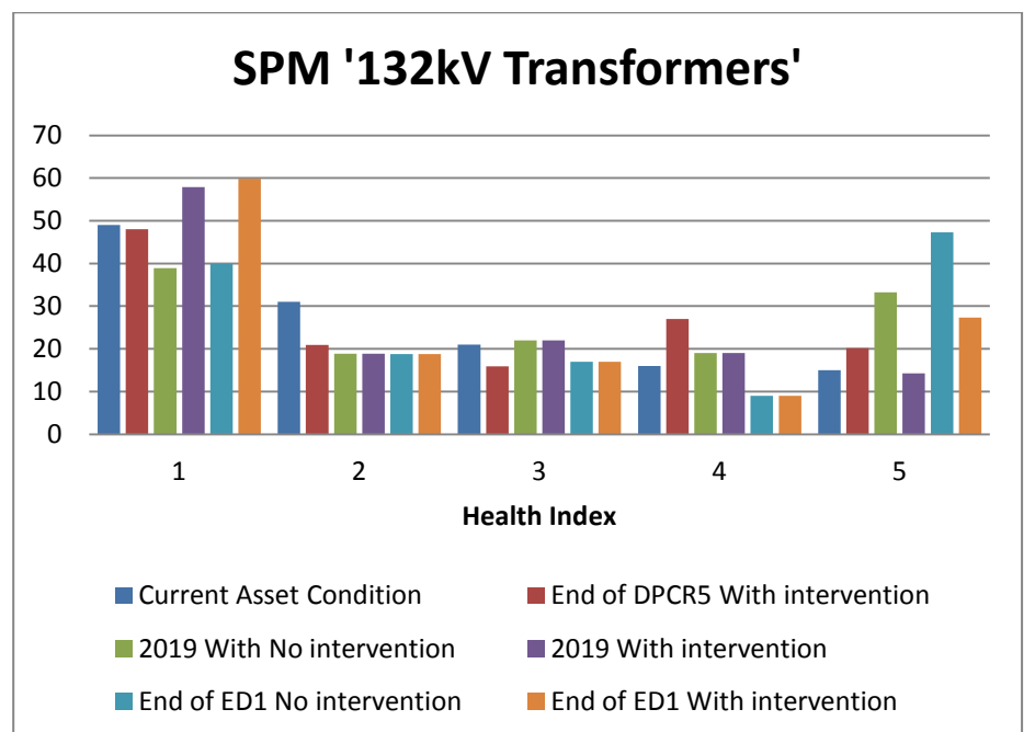
132kV Transformers
