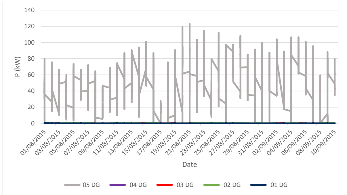
Figure 10: Maximum calculated output of shadow generators in the second case study (descending order)
