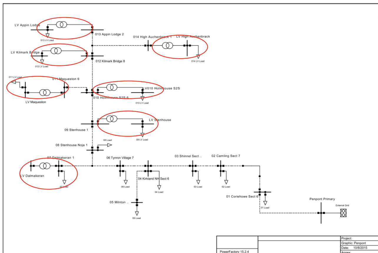
Figure 3: PowerFactory model with LV busbars
