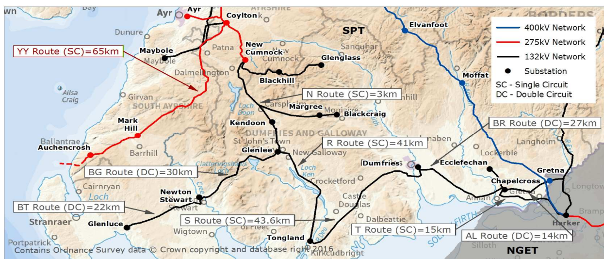
Figure 1: The existing transmission network in Dumfries and Galloway
