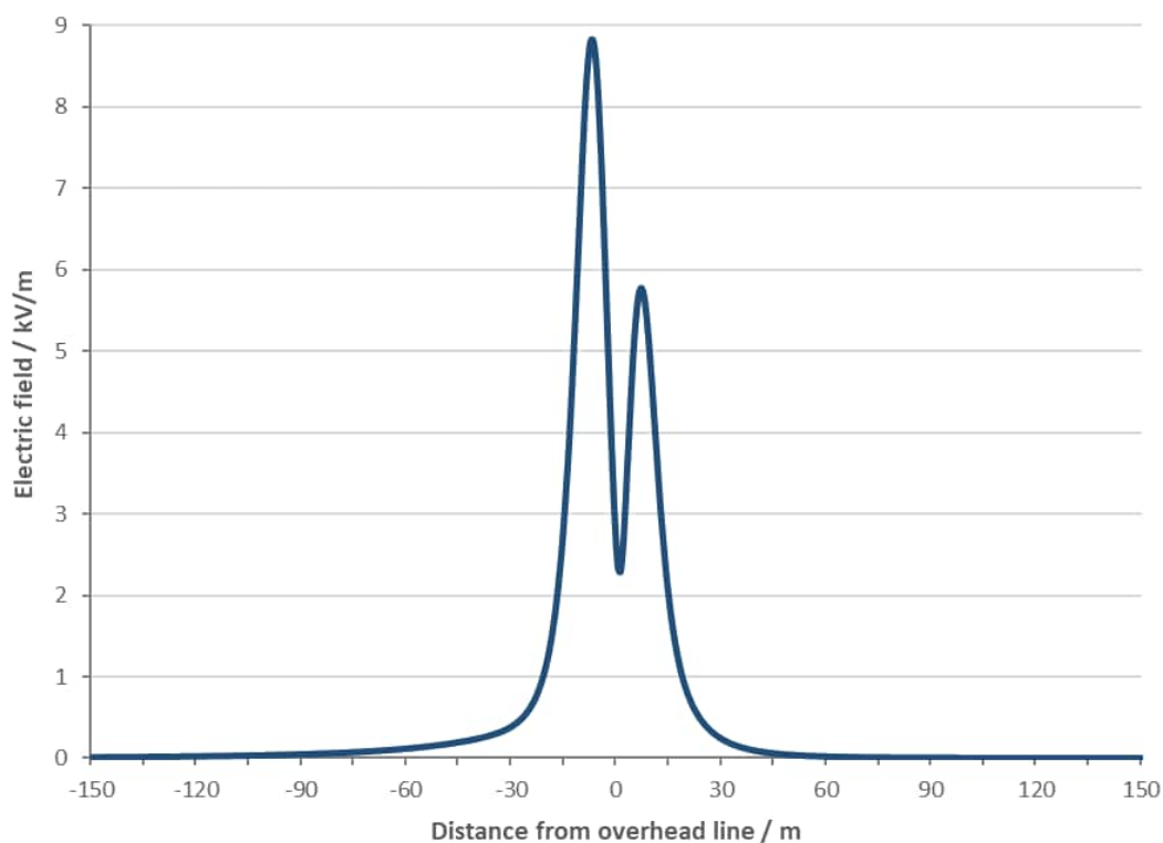
Figure 4.4: Calculated maximum electric fields from XX and XR Overhead Line routes operating at 400/275 kV with Gap conductor system. This represents Options 2 in Table 4.1 which gives the electrical parameters and design information.
