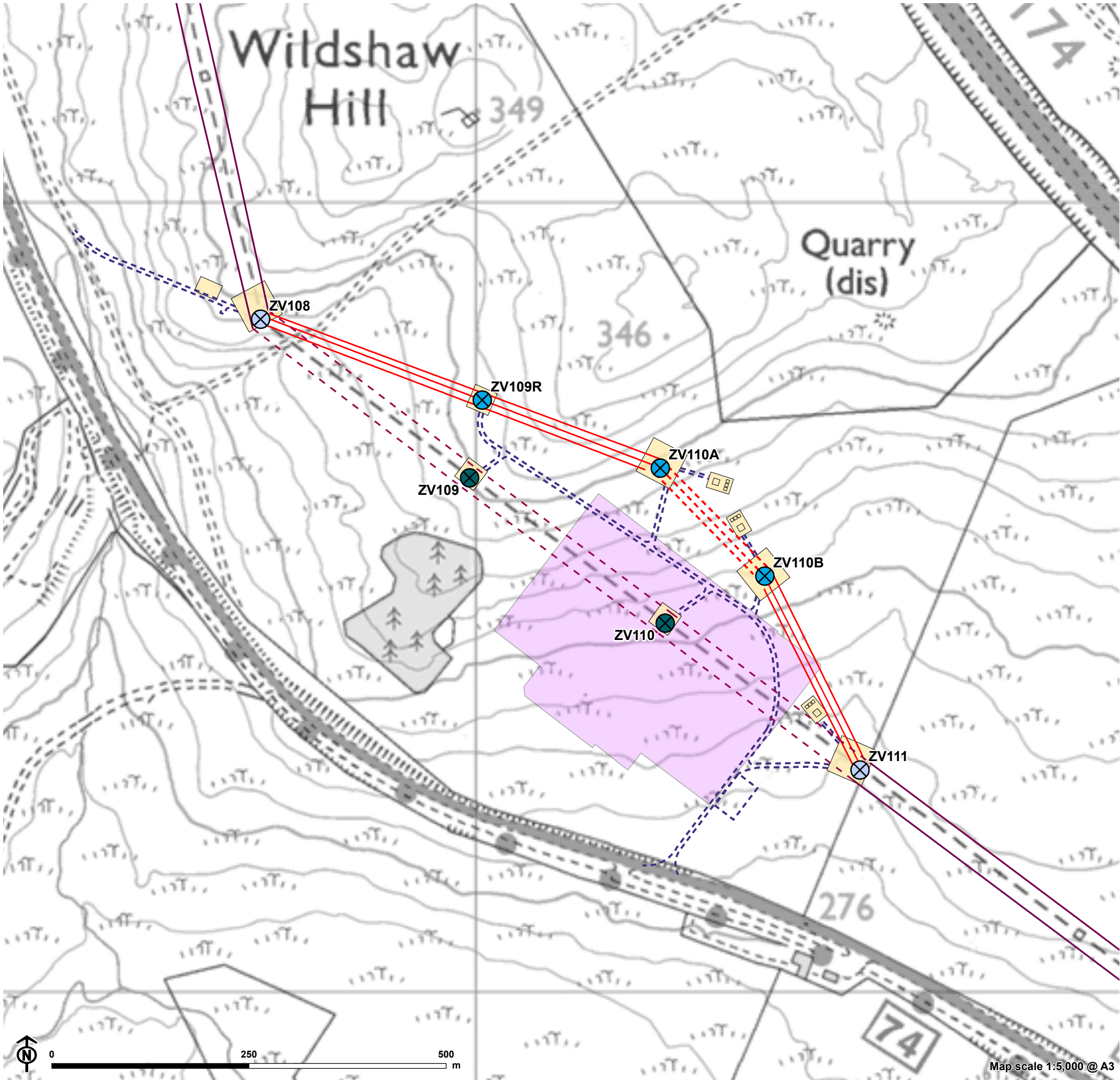
Figure 1.3: Site Plan - Temporary Tower Diversion Proposals
