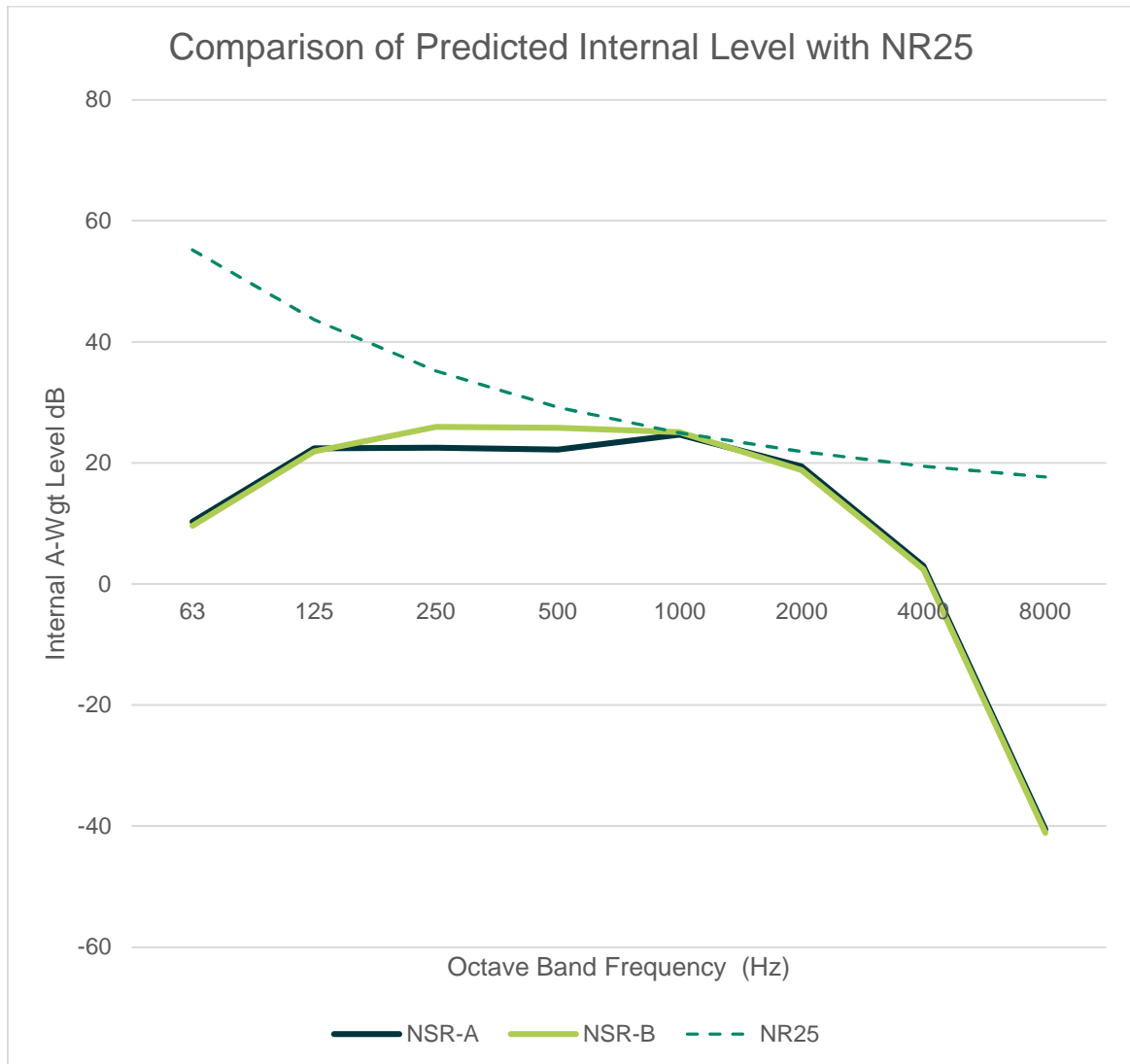
Plate 1 Comparison of predicted internal levels with NR25
