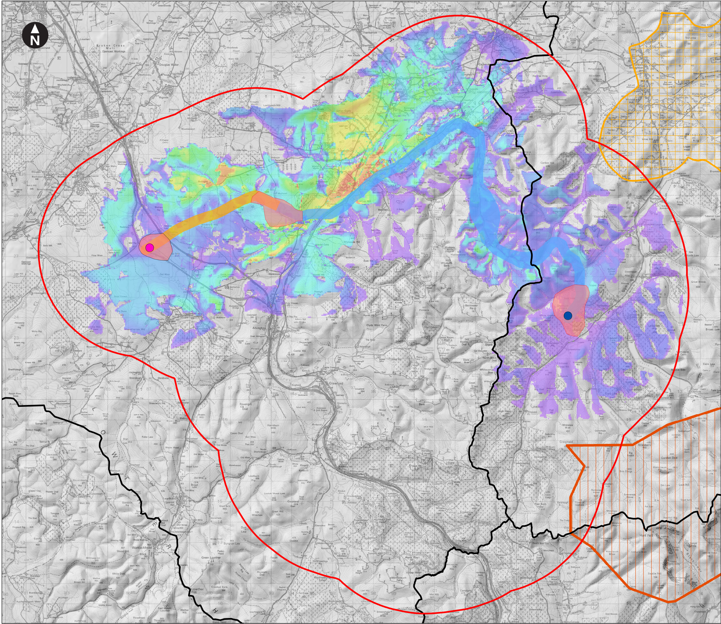
Figure 7.1a Study Area and ZTV - Route Option 1
