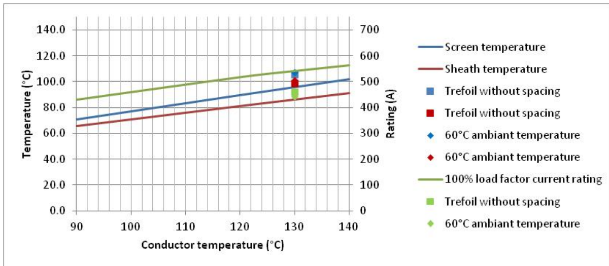
Figure 12 Cable rating calculations for different conductor temperatures, for cables laid in free space. Calculations are based on thermal conductivity data for the blends. Data suggests that at conductor temperature of 140°C (cable rating 564A at 100% load), the sheath temperature is approaching 100°C.
