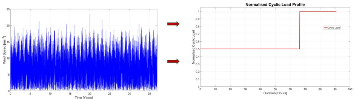
Figure 6 An example of the conversation by the cyclic load profile tool
