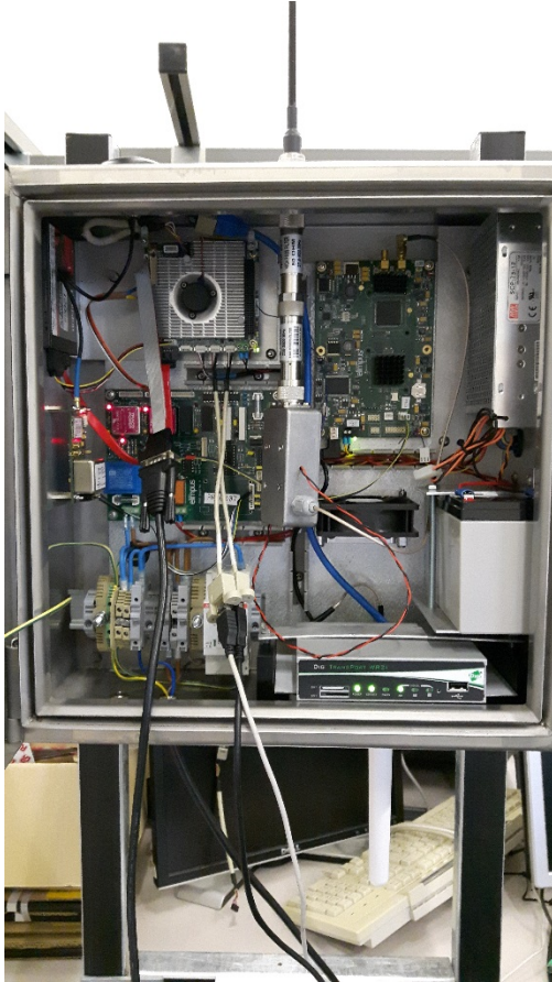
View Inside The RAFL Cabinet
