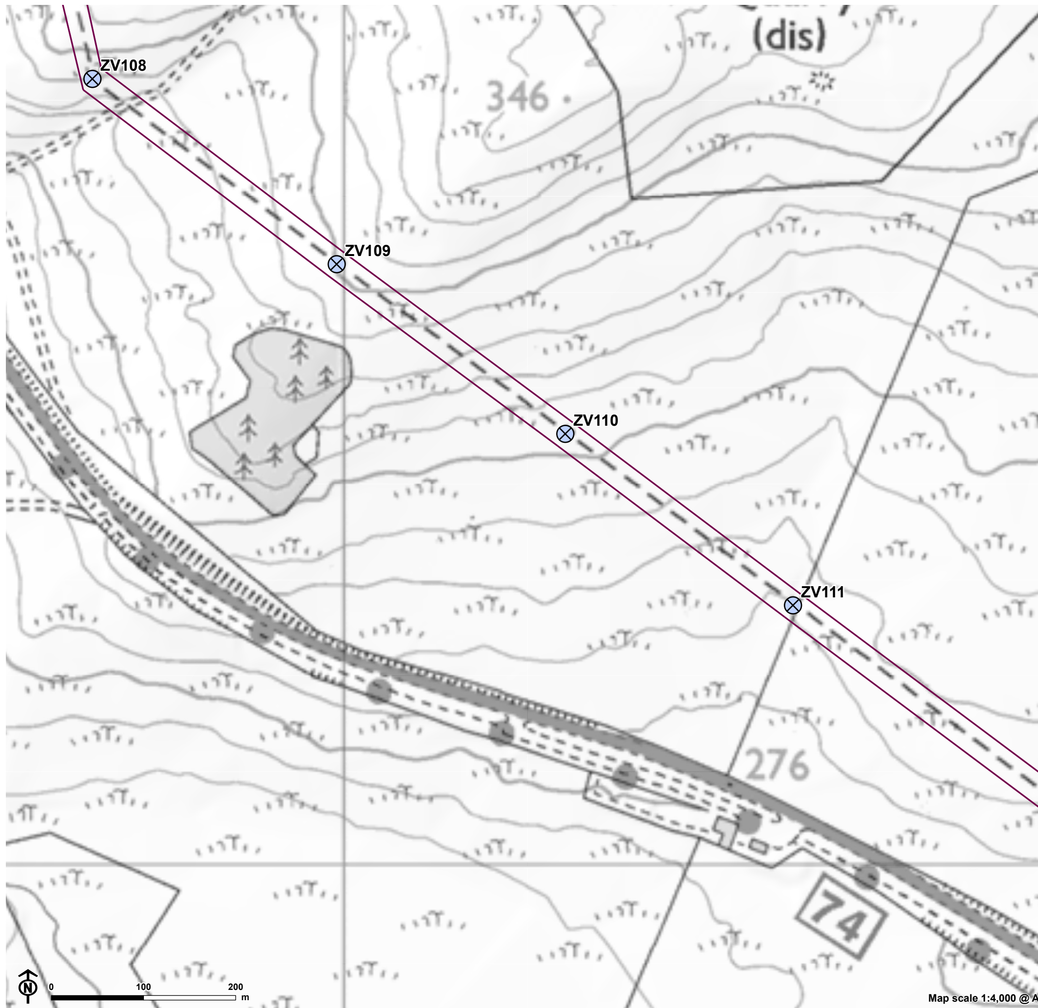
Figure 2.1: General existing site plan
