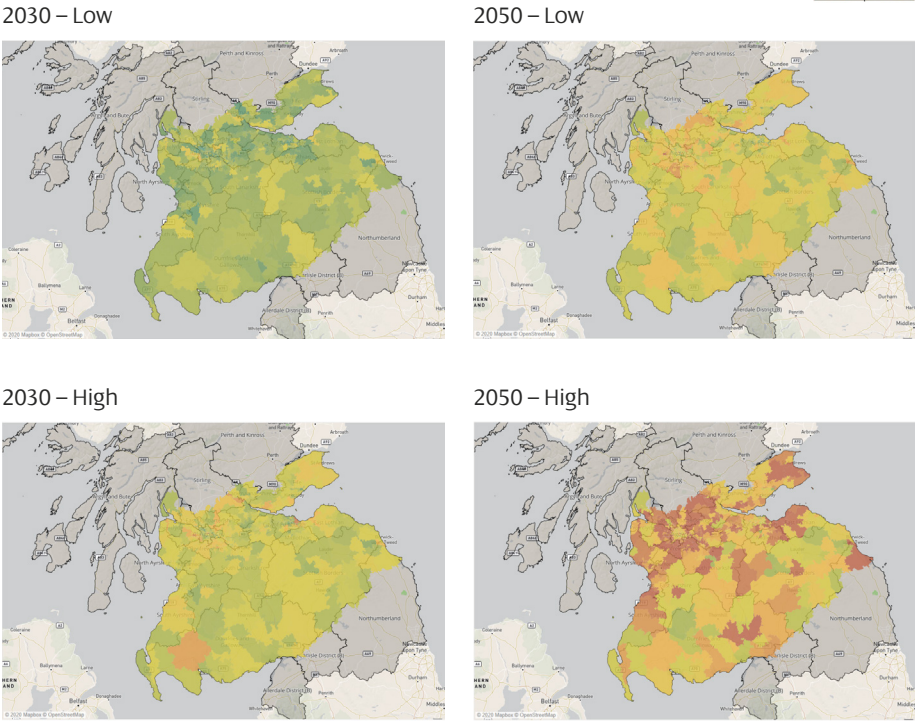
Figure 7 | Electricity peak demand changes from 2019 by primary substation area
