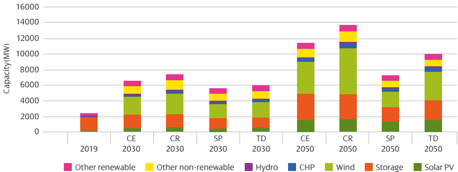
Figure 19 | Breakdown of installed generation capacity by technology type
