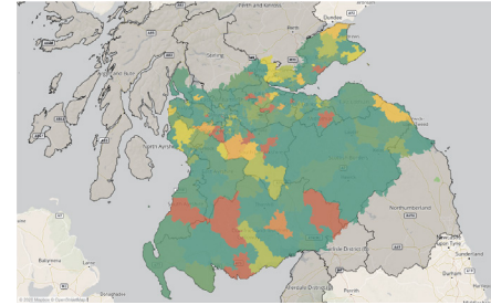
Figure 21 | Domestic-scale and smaller-scale installed generation and storage capacity by primary substation area
