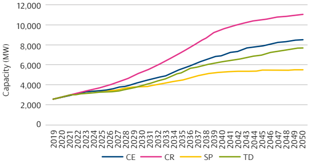
Figure 6 | Total installed generation and storage capacity
