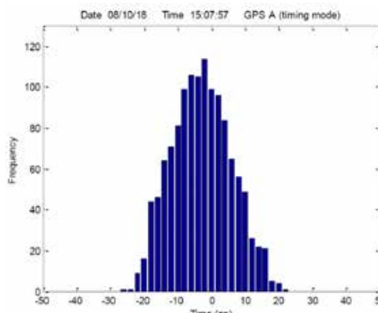
Figure 10 Typical timing accuracy histogram from best performing GPS unit
