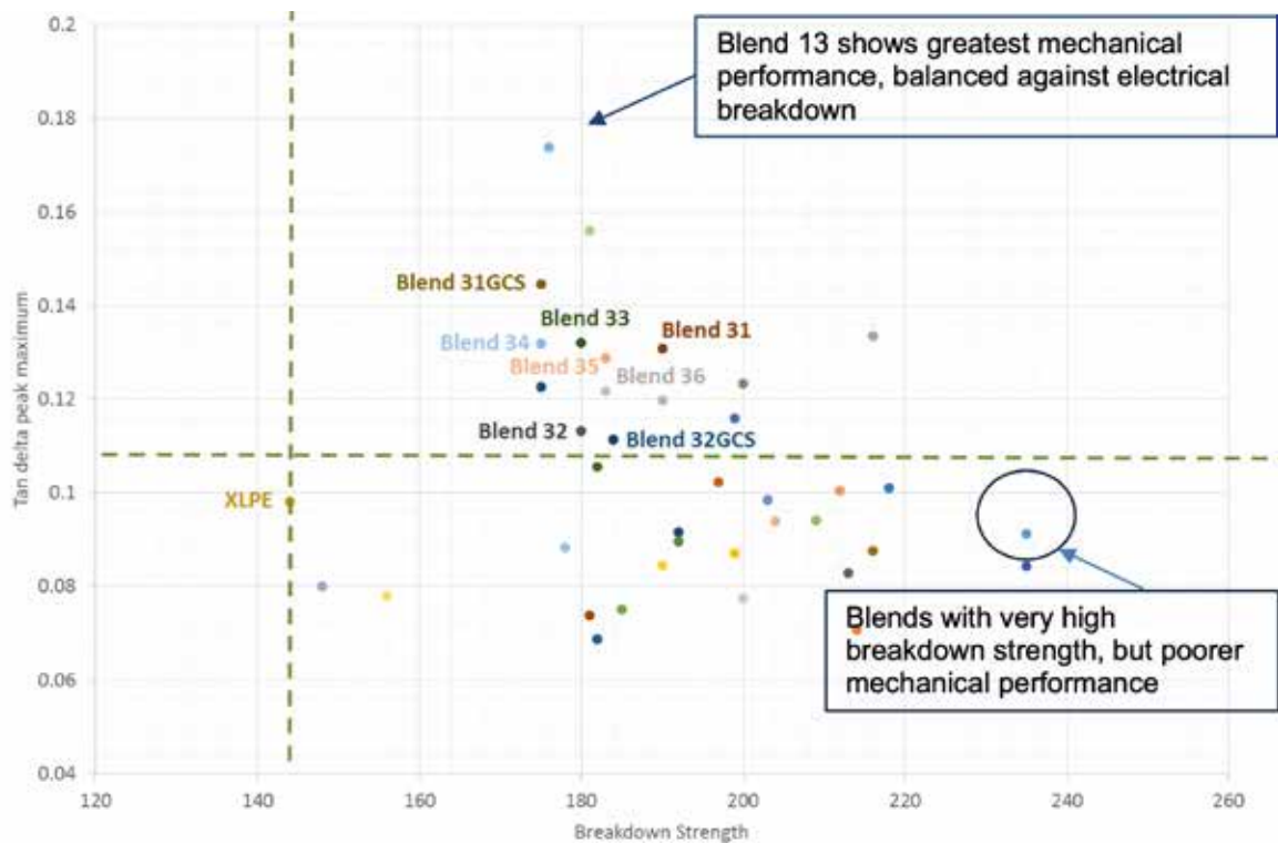
Figure 2 Plot of breakdown strength vs tan delta peak maximum for all blends and XLPE. Dashed lines show the minimum position for both parameters, as achieved by XLPE. Candidate blends for upscaling selected from those towards the top right of the figure.
