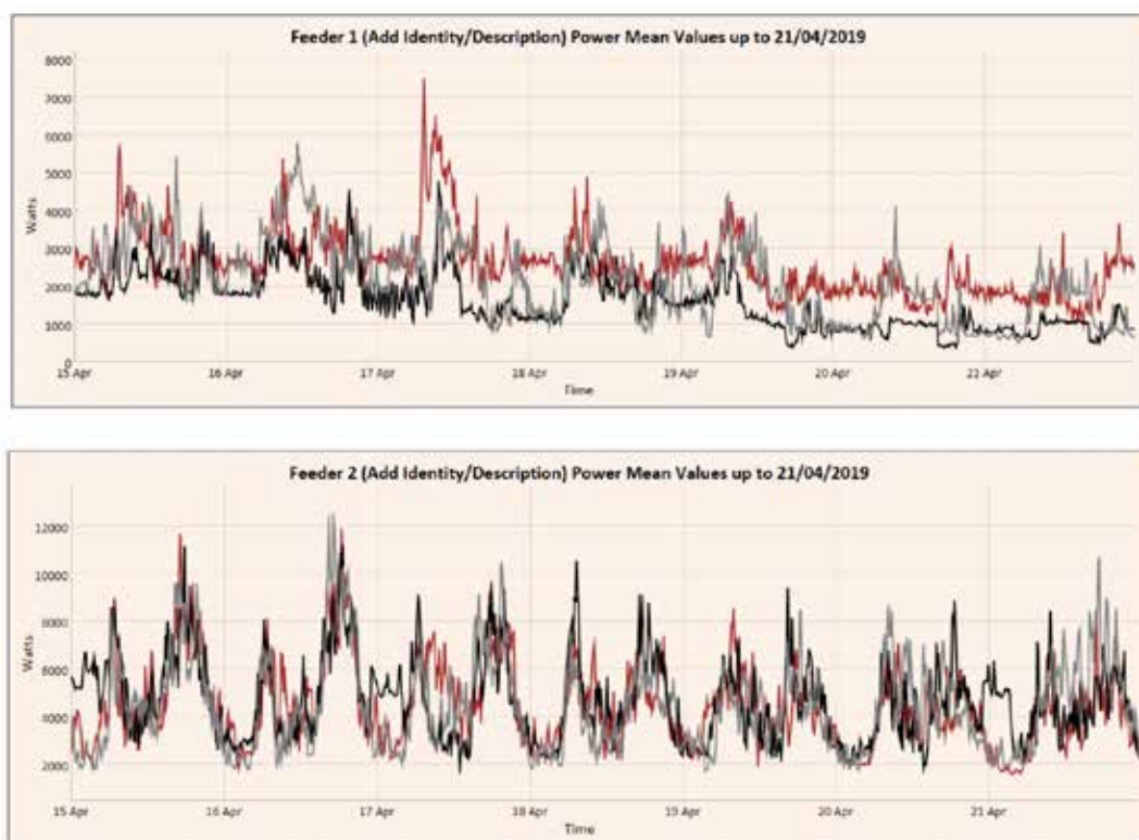
Figure 8 Installation of Heat pump at the new property might have positive impacts on ADMD
