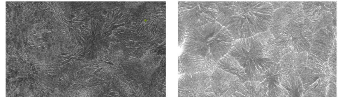
Figure 1 Electron micrographs showing A. a good blend, with no defined borders between spherulites and no evidence of phase separation, B. a poor blend with sharp boundaries between spherulites and evidence of charging (brighter patches)
