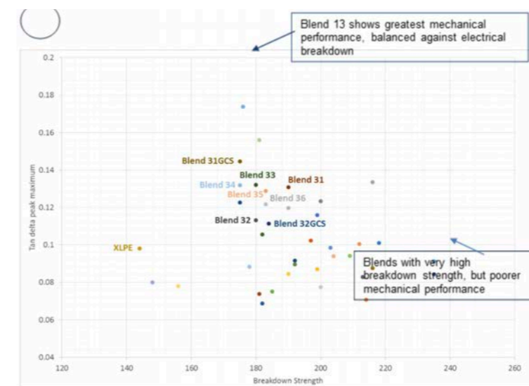
Figure 2 Plot of breakdown strength vs tan delta peak maximum for all blends and XLPE. Dashed lines show the minimum position for both parameters, as achieved by XLPE. Candidate blends for upscaling selected from those towards the top right of the figure.
