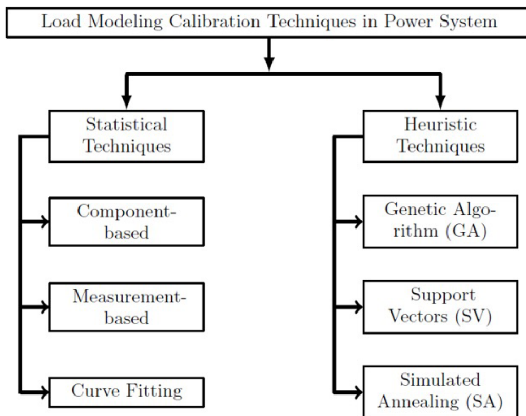
Figure 3: Load Modelling Calibration Techniques
