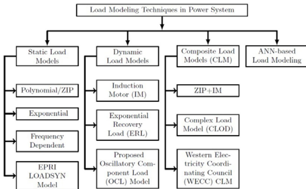
Figure 2: Load Modelling Techniques
