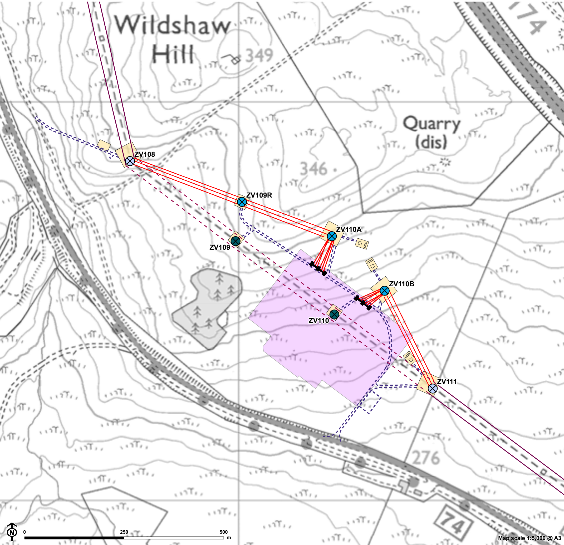
Figure 1.4: Site Plan - Tower Diversion Proposals
