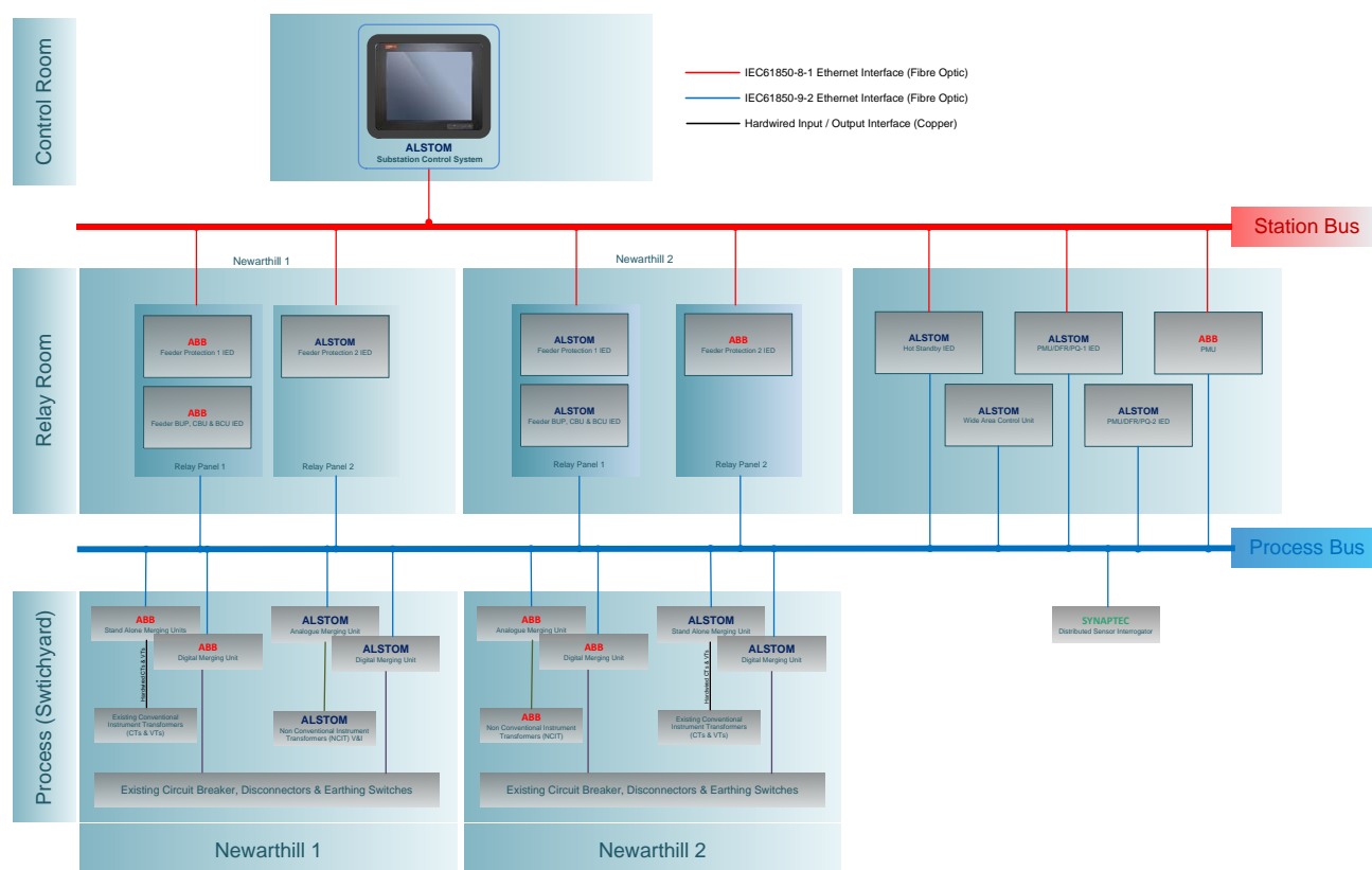
Figure 21 Overview of Proposed Digital Substation Architecture
